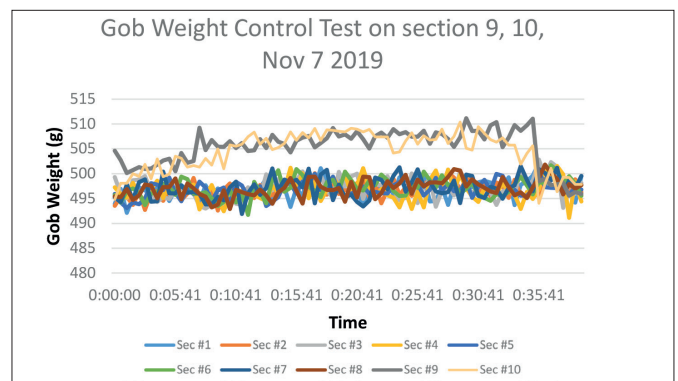
▲ Fig 4. Section 9 and 10 gob weights were set to +10g compared to the others. Their length was set to +3mm compared to the others.
